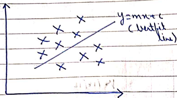
Simple Linear Regression
